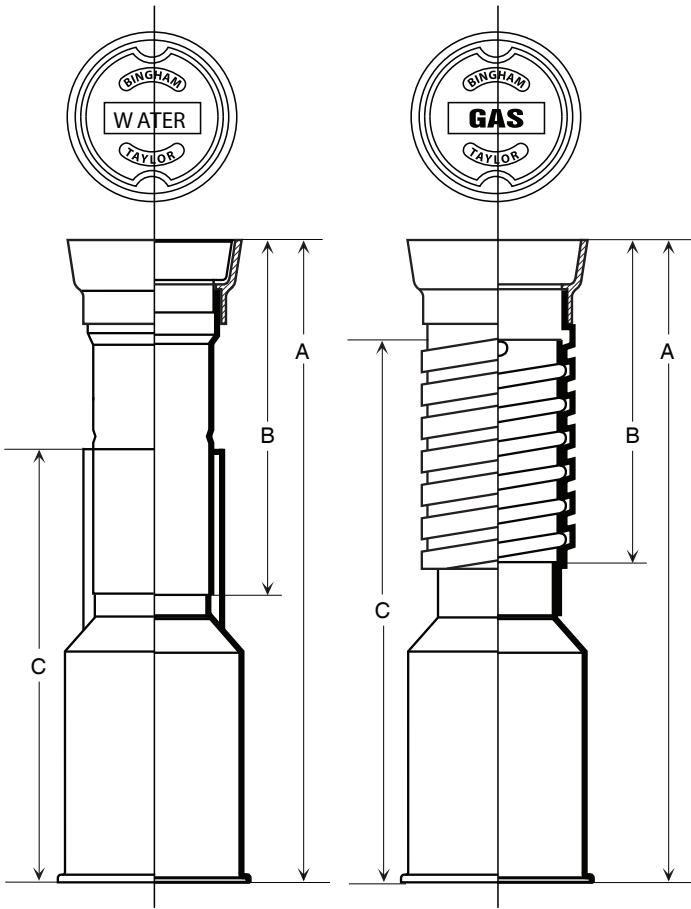
Fig. No. P-500-S Slide Type Box
