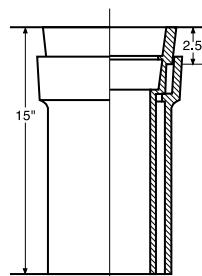
Fig. No. 6020 Sliding Type 15" or 10.5"
