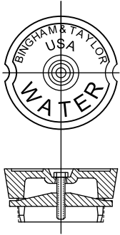
Fig. No. 4904-L Locking Cover
