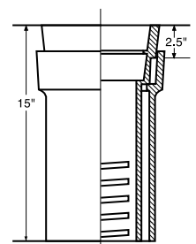
Fig. No. 6030 Screw Type 15"
